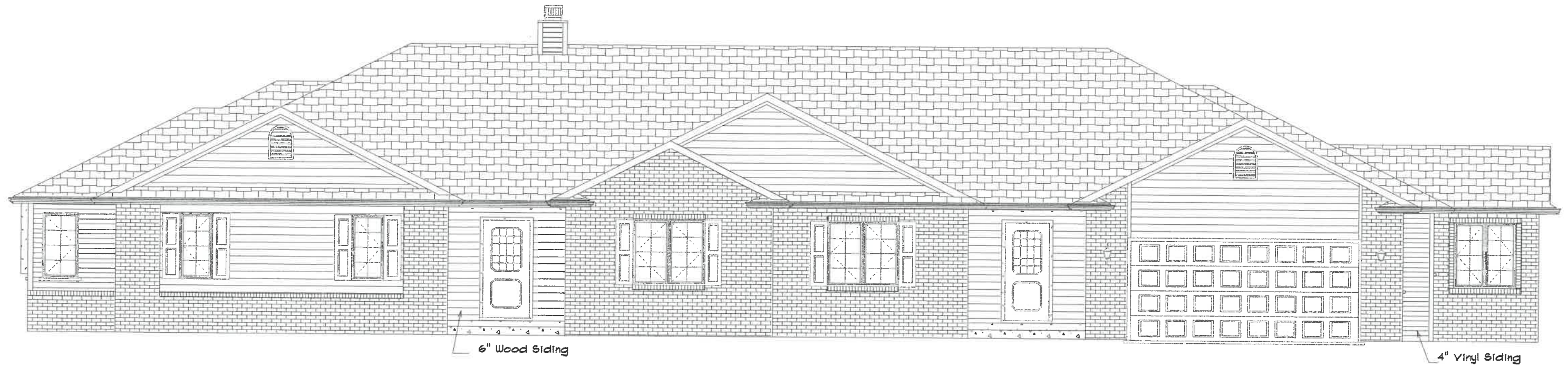
FRONT ELEVATION
