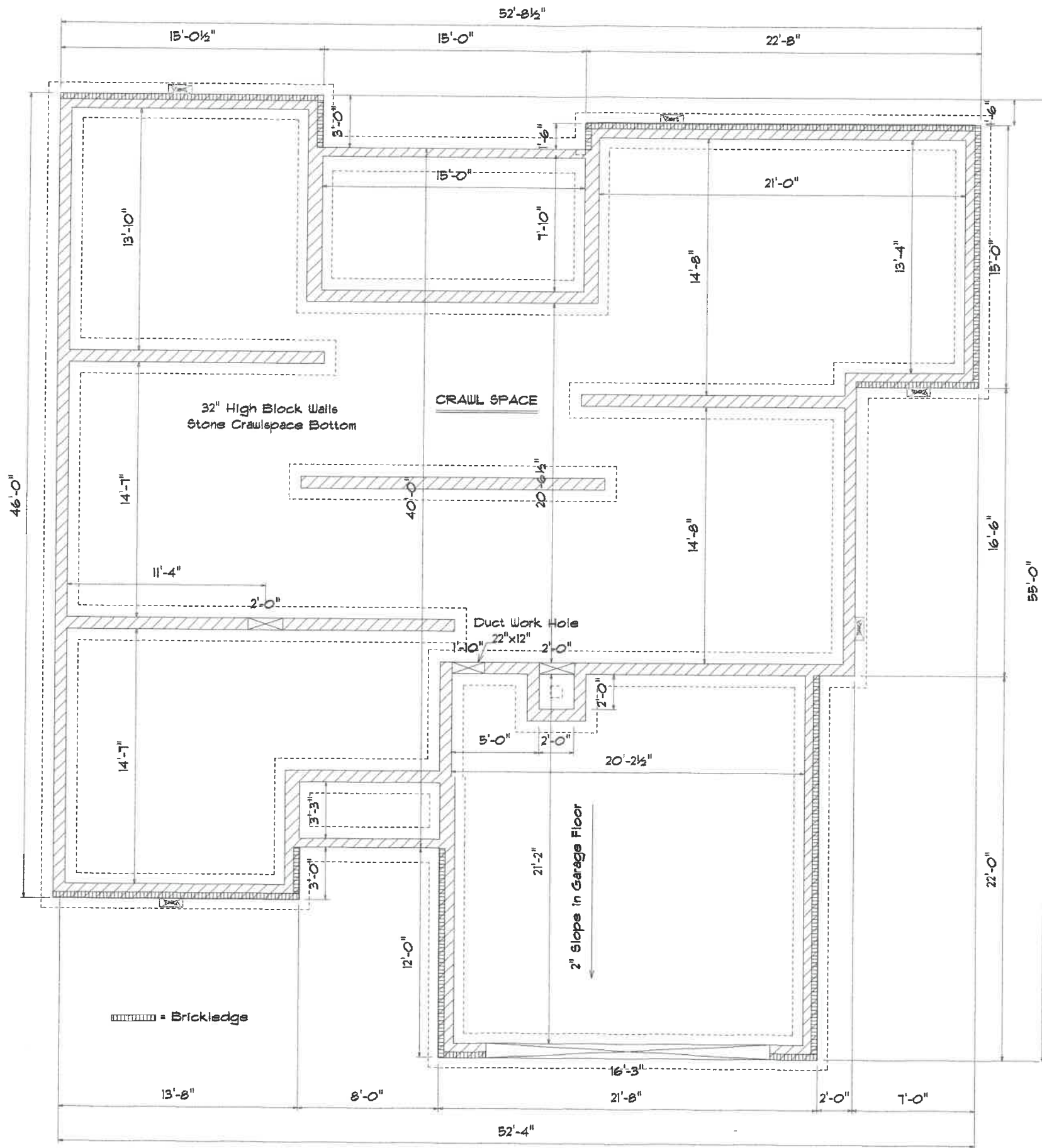
FOUNDATION PLAN
